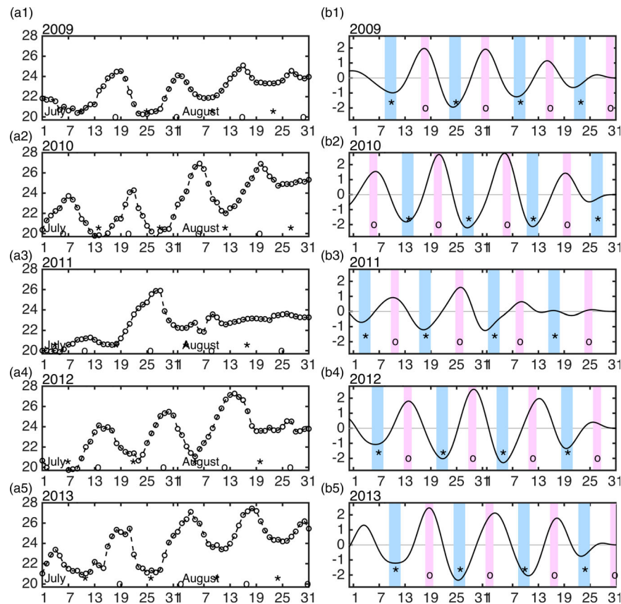
Fig. 7 Time series of modelled temperature ( ^{\circ}\text{C} ) at station A for July and August of 2009–2013. (a) Raw time series and (b) band-pass (7–21 days) filtered time series. The asterisks indicate the times of the spring tide, while the circles mark the times of the neap tide. The blue and red vertical bars in (b) represent the spring and neap tidal phases, respectively.
