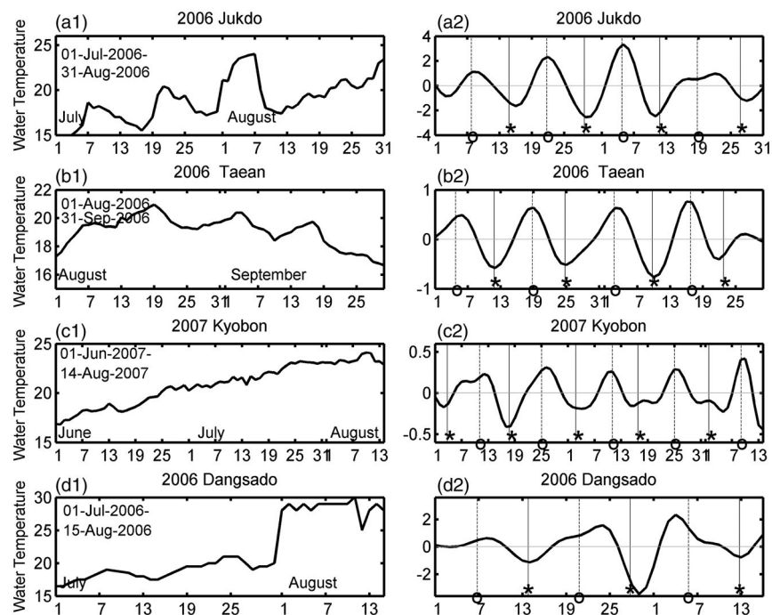
Fig. 18 Raw time series of temperature (°C) from buoy observations at (a1) Jukdo (125.51°E, 34.13°N), (b1) Tae'an (126.24°E, 36.91°N), (c1) Kyobon (128.31°E, 34.70°N), and (d1) Dangsado (126.36°E, 34.05°N). Band-pass filtered (7–21 days) time series of temperature (°C) for (a2) Jukdo, (b2) Tae'an, (c2) Kyobon, and (d2) Dangsado. Asterisks indicate the times of the spring tide, while the circles mark the times of the neap tide. Buoy locations are shown in Fig. 5a.
