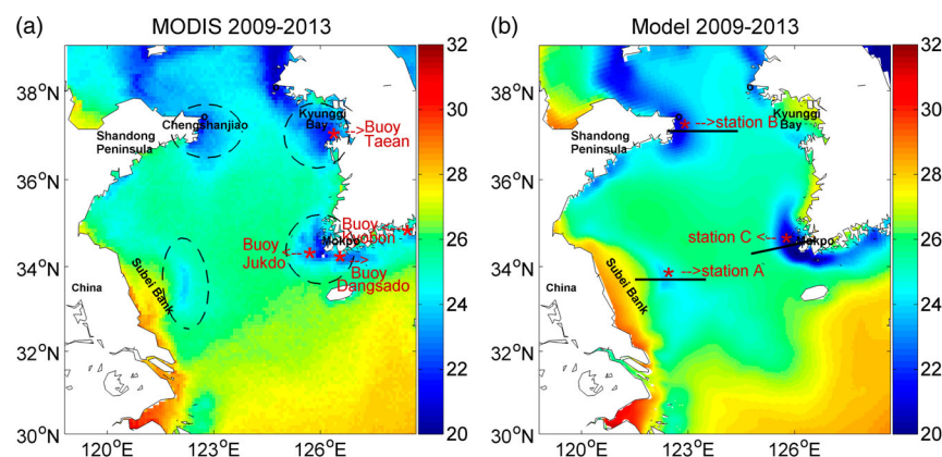
Fig. 5 Distribution of monthly mean SST (°C) for July to August of 2009–2013 from (a) MODIS and (b) model results. The SCPs are marked with dashed ellipses. Locations of stations referred to in Fig. 7 are indicated by asterisks.
